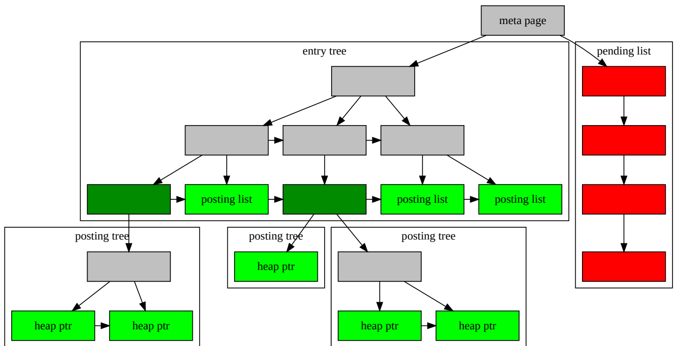
Figure 69.1. GIN Internals
